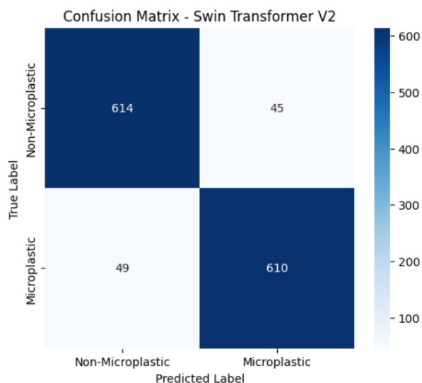
Fig. 6: Confusion Matrix of Swin Transformer V2
