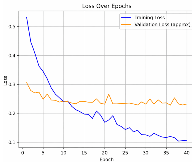
Fig. 8: Training and Validation loss Trend Across 40 Epochs Using Swin Transformer V2
