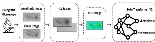
Fig. 1: Block Diagram of the Proposed Swin Transfer V2 Architecture.
