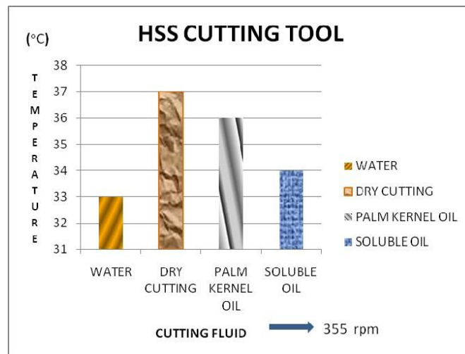
Fig 2: Graph of temperature variation during cutting and cooling for HSS cutting tool
