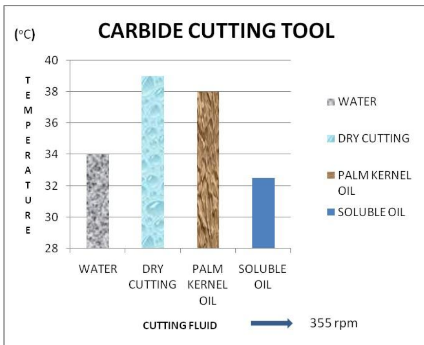
Fig 3: Graph of temperature variation during cutting and cooling for carbide cutting tool
